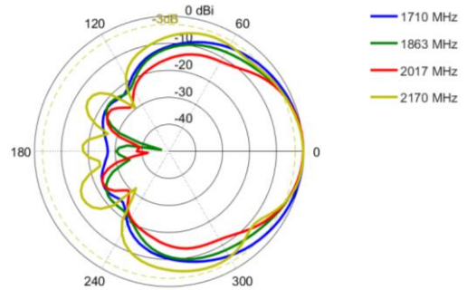
Azimuth (Top View): 1710 – 2170 MHz
