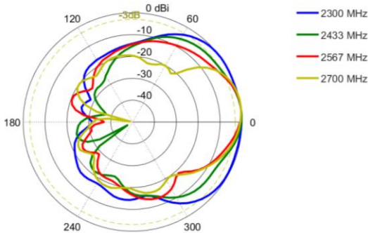
Elevation (Side View): 2300 – 2700 MHz
