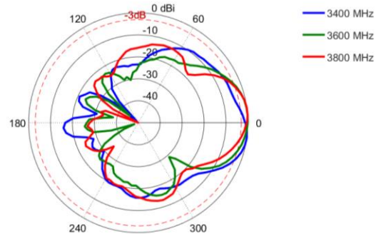
Elevation (Side View): 3400 – 3800 MHz
