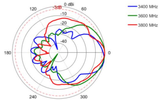
Azimuth (Top View): 3400 – 3800 MHz
